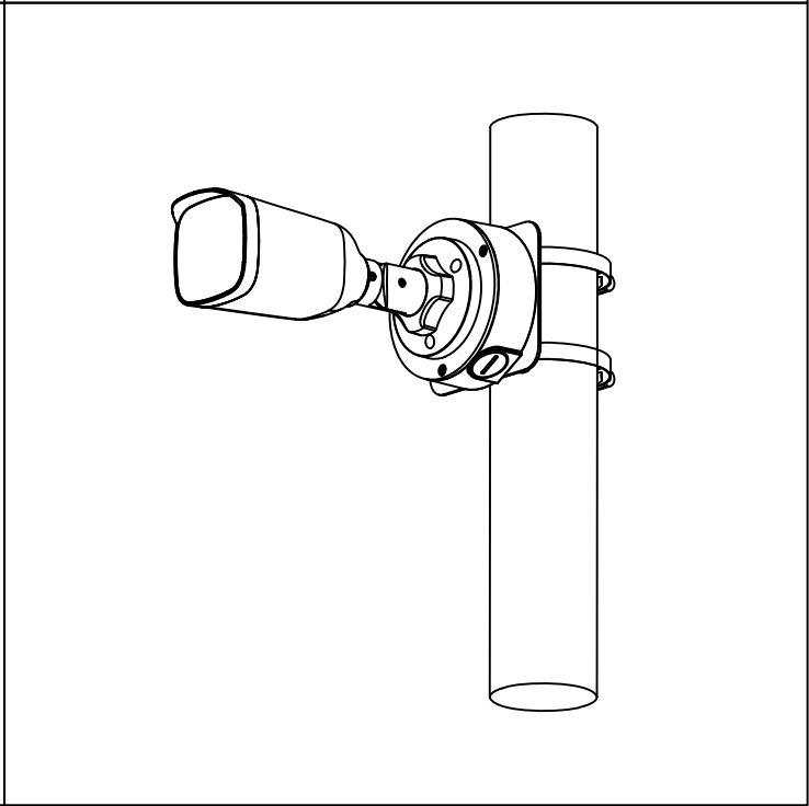
Pole Mount(Vertical)
