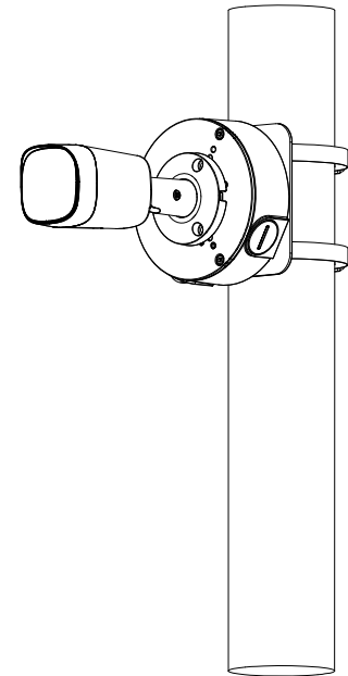
Pole Mount(Vertical)
