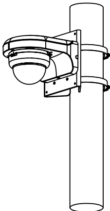
Pole Mount(Vertical)
