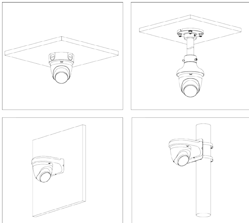
Figure 4-3 Installation method
