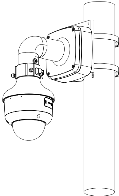
Pole Mount(Vertical)
