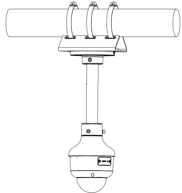
Pole Mount(Horizontal)
